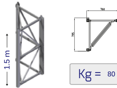
Traliccio triangolare Triangular mast / Mât triangulaire
